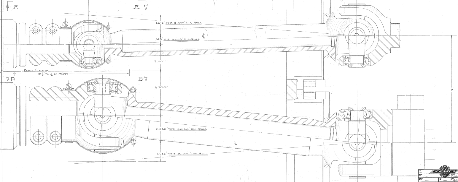
VIEW-AA
