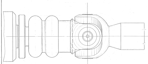
VIEW-AA
